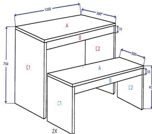
Zaagplan picknickset
